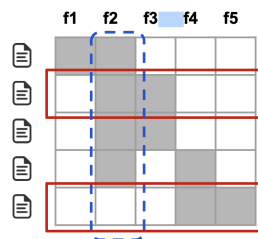
Figure 1: Explanation Matrix : SubModular Pick Algorithm
