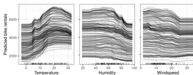
Figure 3: Examples of ICE Plots
